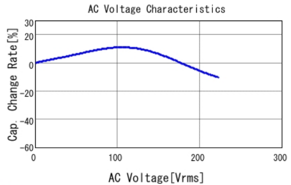
■ GCJ32DR72J473KXJ1 C-AC Voltage capchange, DC0V, 25.0d
