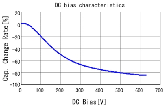
■ GCJ32DR72J473KXJ1 C-DC bias capchange, 25.0degC, AC1V
