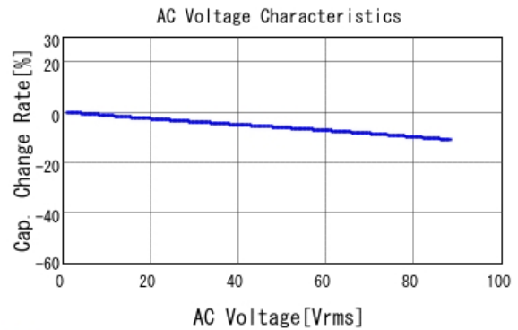
■ GCJ32DR72E224KXJ1 C-AC Voltage capchange, DC0V, 25.0d
