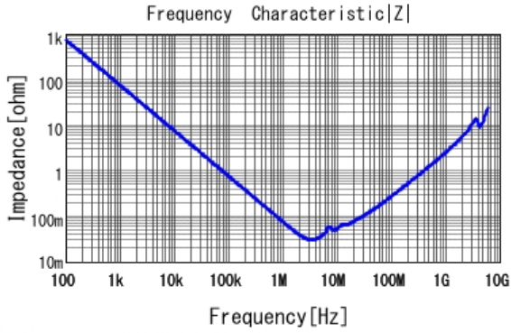
■ GCJ32DR72A225MA01 |Z| DC0V, 25degC
