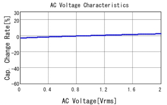
■ GCJ32DR72A225MA01 C-AC Voltage capchange, DC0V, 25.0d
