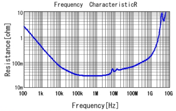
■ GCJ32DR72A225MA01 R DC0V, 25degC
