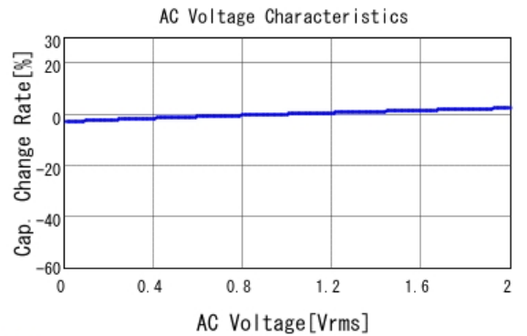
■ GCJ32DL8EL225KA07 C-AC Voltage capchange, DC0V, 25.0d
