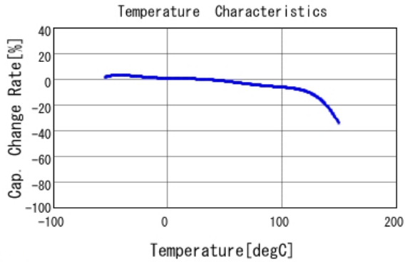
■ GCJ32DL8EL225KA07 C-Temp. capchange, DC0.0V, AC1.0V rm
