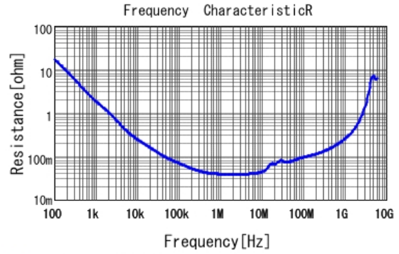
■ GCJ31MR71H474KA01 R DCOV, 25degC
