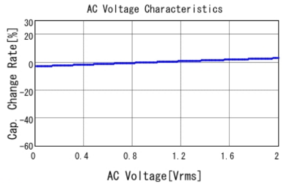
■ GCJ31MR71H474KA01 C-AC Voltage capchange, DCOV, 25.0d
