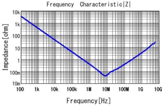
■ GCJ31MR71H474KA01 |Z| DCOV, 25degC
