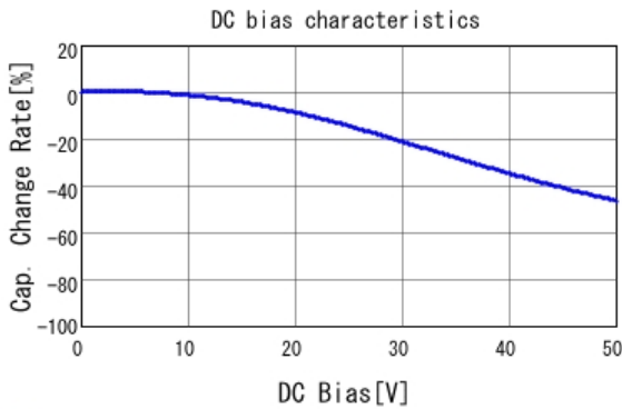
■ GCJ31MR71H474KA01 C-DC bias capchange, 25.0degC, AC1.
