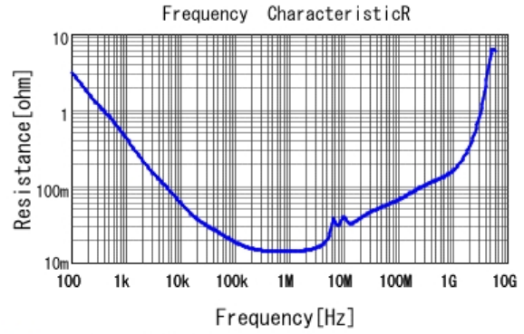
■ GCJ31CR71H225MA12 R DC0V, 25degC
