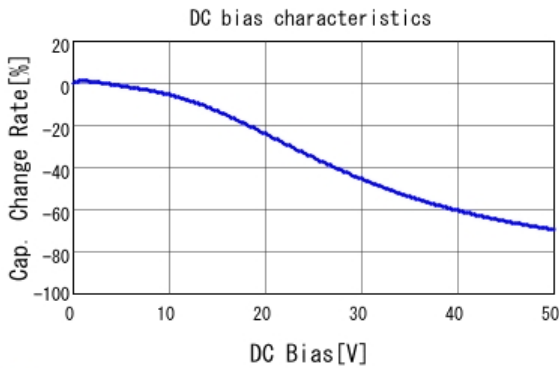
■ GCJ31CR71H225MA12 C-DC bias capchange, 25.0degC, AC1.
