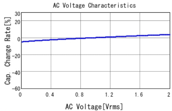
■ GCJ31CR71H225MA12 C-AC Voltage capchange, DC0V, 25.0d
