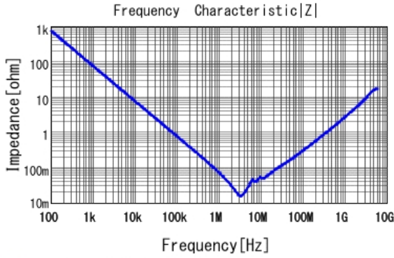
■ GCJ31CR71H225MA12 |Z| DC0V, 25degC
