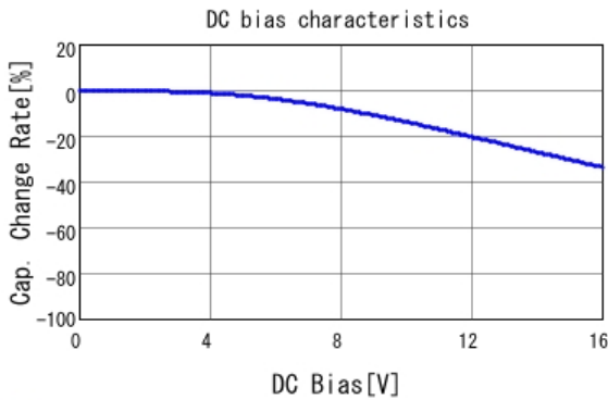
■ GCJ31CR71C475KA01 C-DC bias capchange, 25.0degC, AC1.
