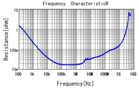
■ GCJ31CR71C475KA01 R DC0V, 25degC
