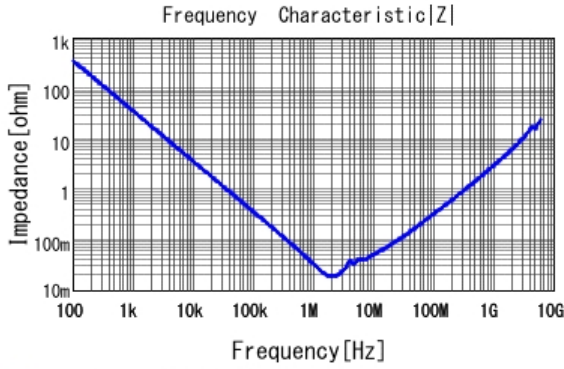
■ GCJ31CR71C475KA01 |Z| DC0V, 25degC
