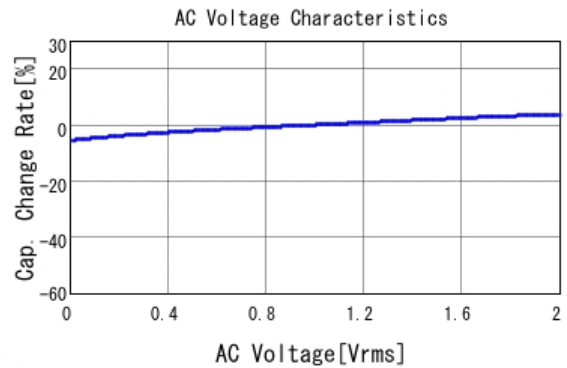
■ GCJ31CR71C475KA01 C-AC Voltage capchange, DC0V, 25.0d
