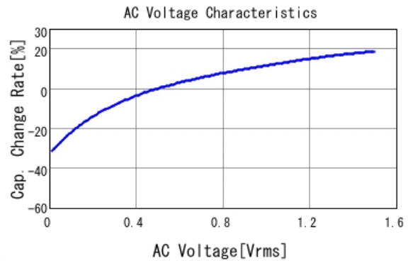
■ GCJ31CR71A226KE01 C-AC Voltage capchange, DC0V, 25.0d
