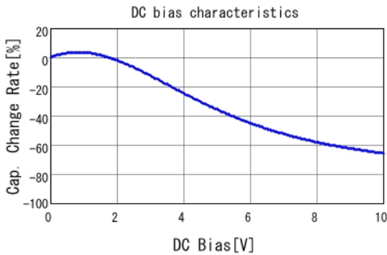
■ GCJ31CR71A226KE01 C-DC bias capchange, 25.0degC, AC0.
