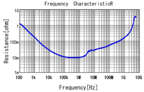
■ GCJ31CC71H475MA01 R DC0V, 25degC
