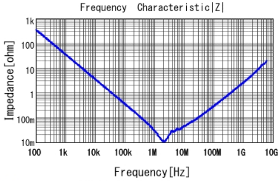
■ GCJ31CC71H475MA01 |Z| DC0V, 25degC
