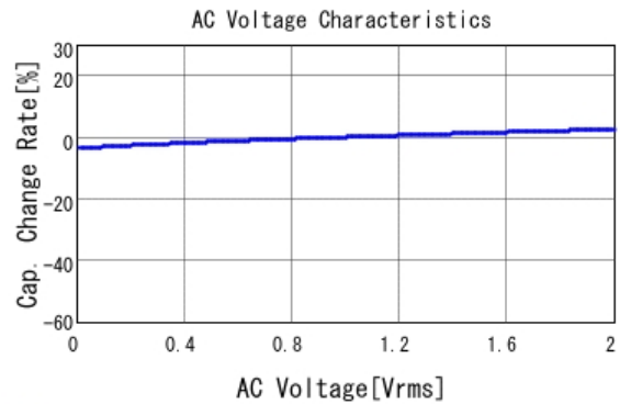
■ GCJ31CC71H475MA01 C-AC Voltage capchange, DC0V, 25.0d
