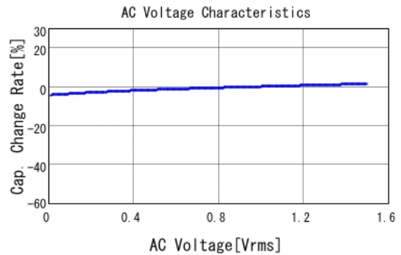
■ GCJ31CC71E106MA15 C-AC Voltage capchange, DCOV, 25.0d
