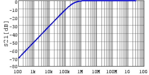
GCJ31BR73A472KXJ1 S21 DC0V,25degC
