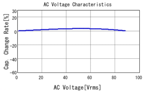
■ GCJ21BR72E153KXJ3 C-AC Voltage capchange, DC0V, 25.0d
