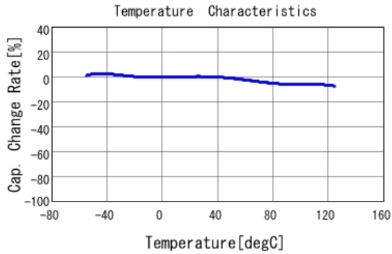
■ GCJ21BR71H473KA01 C-Temp. capchange, DC0.0V, AC1.0Vrm
