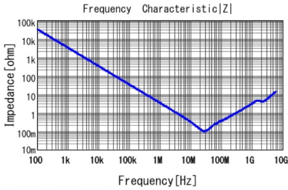
■ GCJ21BR71H473KA01 |Z| DCOV, 25degC
