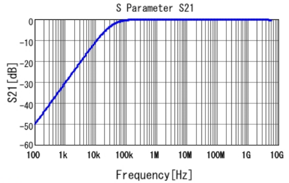
■ GCJ21BR71H473KA01 S21 DC0V, 25degC
