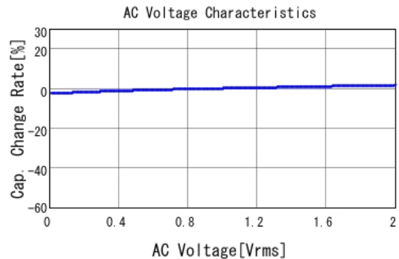
■ GCJ21BR71H473KA01 C-AC Voltage capchange, DCOV, 25.0d
