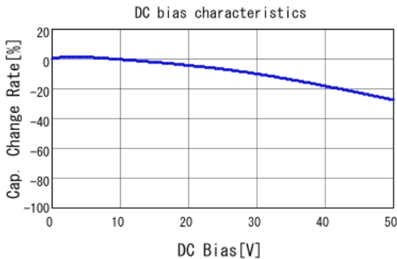
■ GCJ21BR71H473KA01 C-DC bias capchange, 25.0degC, AC1.
