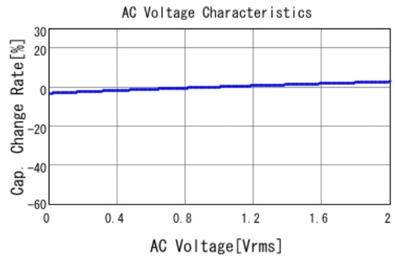
■ GCJ21BR71H224MA01 C-AC Voltage capchange, DCOV, 25.0d
