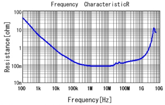
■ GCJ21BR71H224MA01 R DCOV, 25degC
