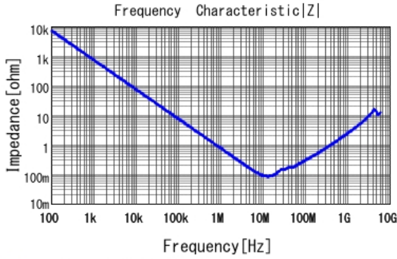
■ GCJ21BR71H224MA01 |Z| DCOV, 25degC
