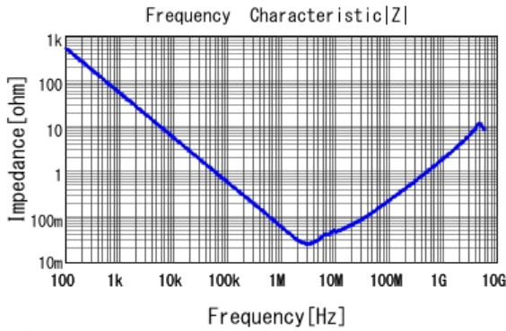
■ GCJ21BR71C475MA01 |Z| DCOV, 25degC
