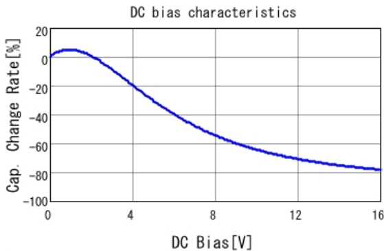
■ GCJ21BR71C475MA01 C-DC bias capchange, 25.0degC, AC1.
