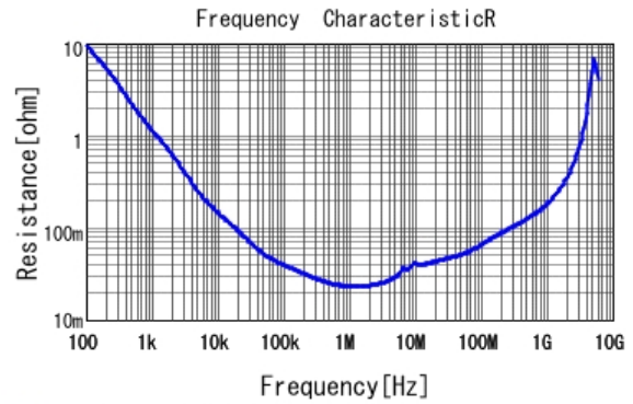
■ GCJ21BR71C475MA01 R DCOV, 25degC
