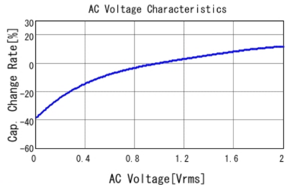
■ GCJ21BR71C475MA01 C-AC Voltage capchange, DCOV, 25.0d
