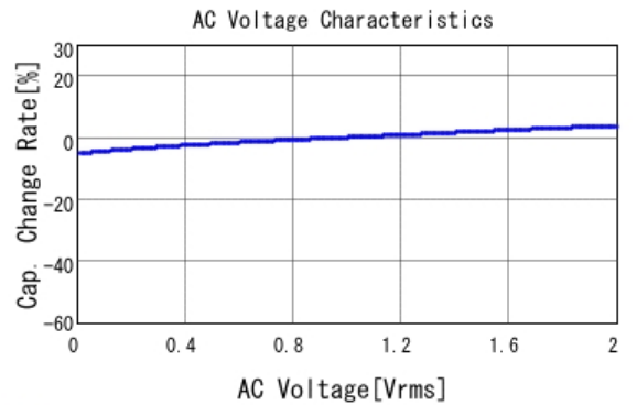
■ GCJ21BR71C105KA01 C-AC Voltage capchange, DCOV, 25.0d
