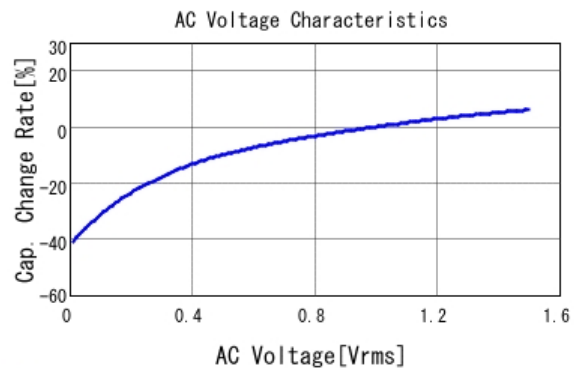
■ GCJ21BR71A106KE01 C-AC Voltage capchange, DC0V, 25.0d
