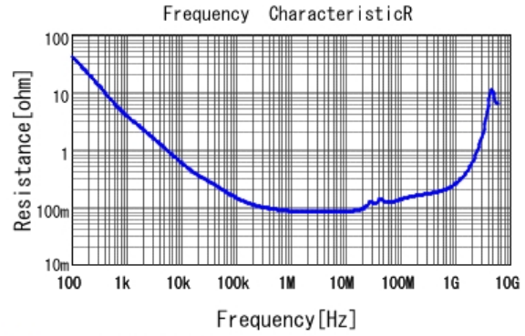
■ GCJ21BL8YA224KA01 R DC0V, 25degC
