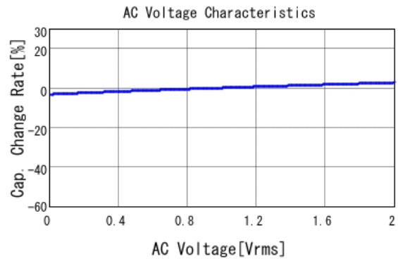
■ GCJ21BL8YA224KA01 C-AC Voltage capchange, DC0V, 25.0d
