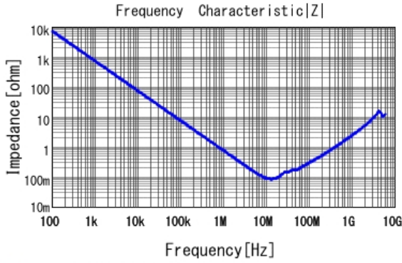
■ GCJ21BL8YA224KA01 |Z| DC0V, 25degC
