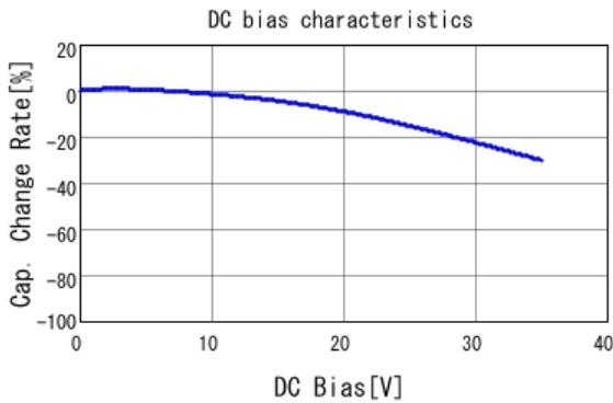
■ GCJ21BL8YA224KA01 C-DC bias capchange, 25.0degC, AC1.
