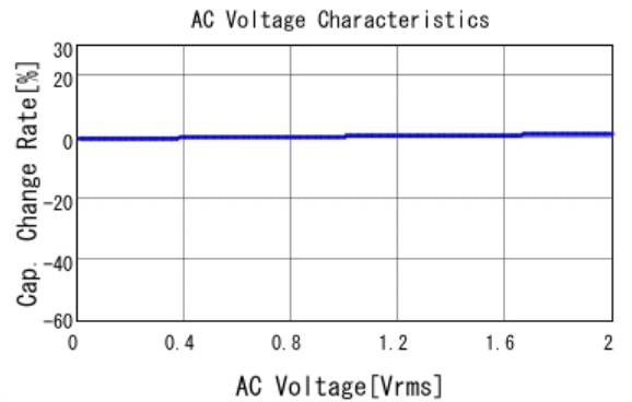
■ GCJ219R72A471KA01 C-AC Voltage capchange, DCOV, 25.0d
