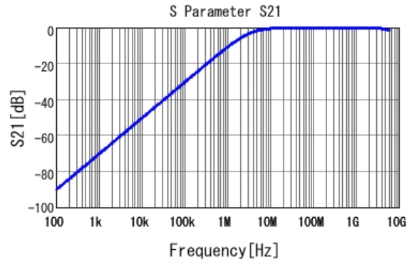
■ GCJ219R72A471KA01 S21 DC0V, 25degC
