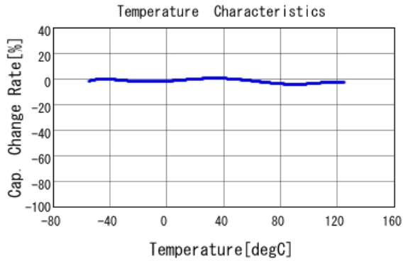
■ GCJ219R72A471KA01 C-Temp. capchange, DC0.0V, AC1.0Vrm
