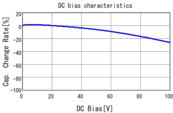
■ GCJ216R72A222KA01 C-DC bias capchange, 25.0degC, AC1.
