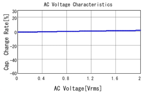
■ GCJ216R72A222KA01 C-AC Voltage capchange, DCOV, 25.0d
