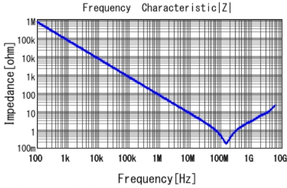
■ GCJ216R72A222KA01 |Z| DCOV, 25degC
