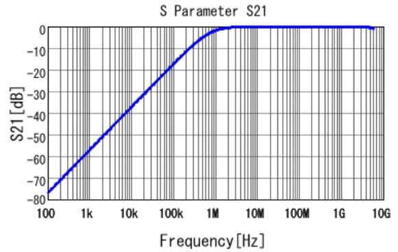
■ GCJ216R72A222KA01 S21 DC0V, 25degC
