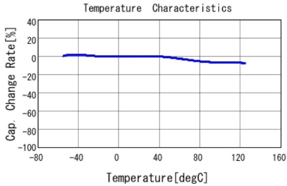
■ GCJ216R72A222KA01 C-Temp. capchange, DC0.0V, AC1.0Vrm
