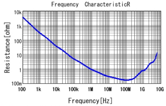
■ GCJ216R72A222KA01 R DCOV, 25degC
