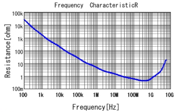
■ GCJ216R71H471KA01 R DCOV, 25degC
