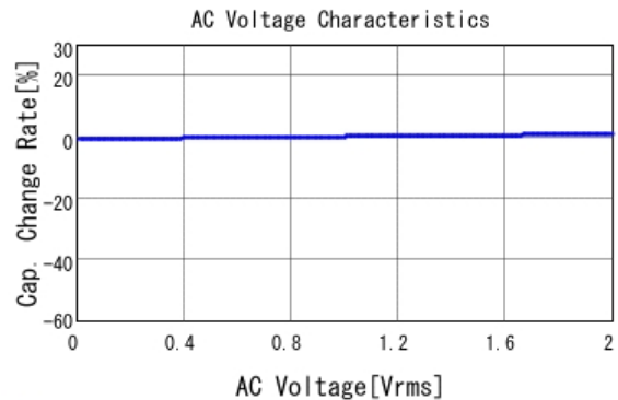
■ GCJ216R71H471KA01 C-AC Voltage capchange, DCOV, 25.0d
