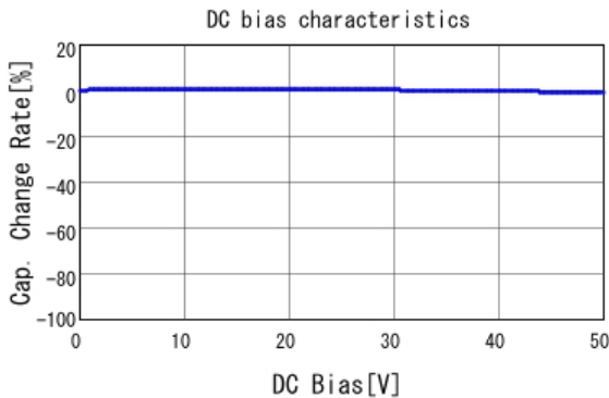
■ GCJ216R71H471KA01 C-DC bias capchange, 25.0degC, AC1.
