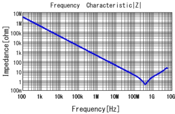
■ GCJ216R71H471KA01 |Z| DCOV, 25degC
