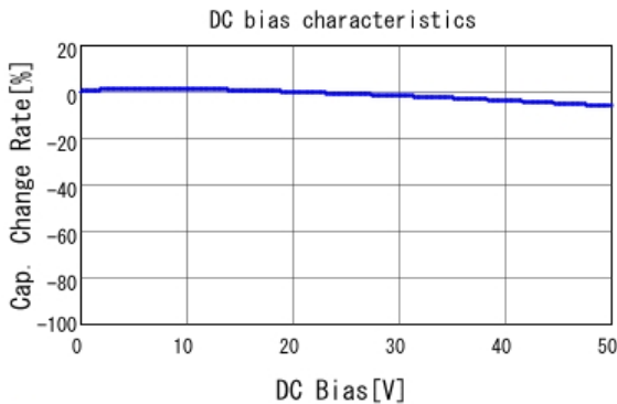
■ GCJ216R71H222KA01 C-DC bias capchange, 25.0degC, AC1.
