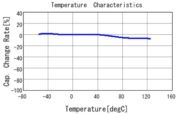
■ GCJ216R71H222KA01 C-Temp. capchange, DC0.0V, AC1.0Vrm
