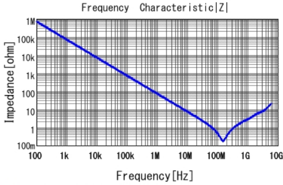
■ GCJ216R71H222KA01 |Z| DCOV, 25degC
