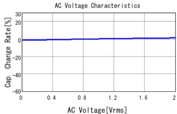
■ GCJ216R71H222KA01 C-AC Voltage capchange, DCOV, 25.0d
