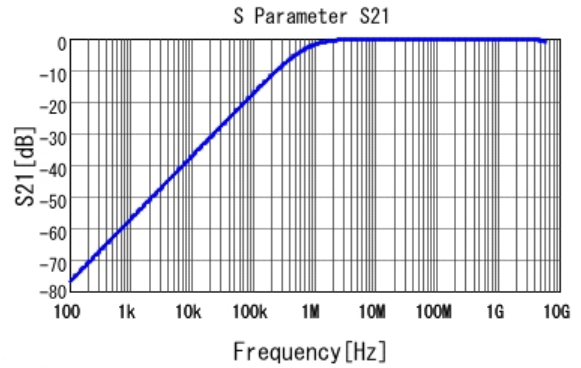
■ GCJ216R71H222KA01 S21 DC0V, 25degC
