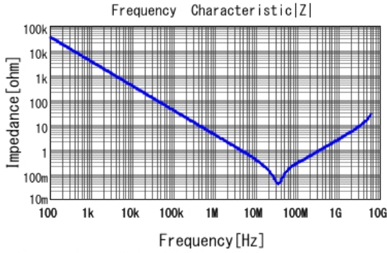
■ GCJ188R92A473MA01 |Z| DCOV, 25degC
