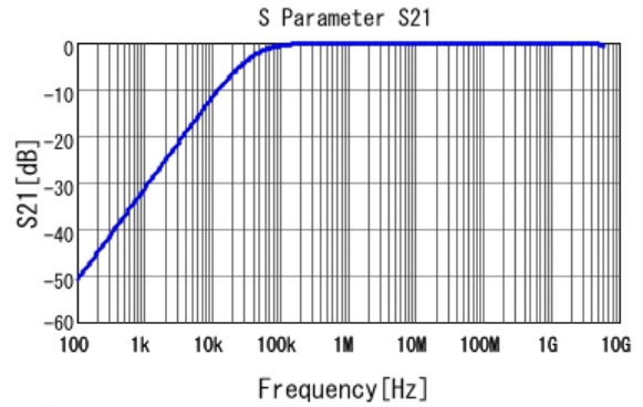
■ GCJ188R92A473MA01 S21 DC0V, 25degC
