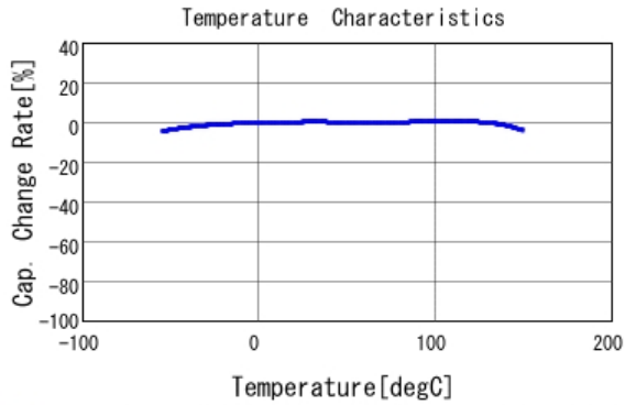
■ GCJ188R92A473MA01 C-Temp. capchange, DC0.0V, AC1.0Vrm
