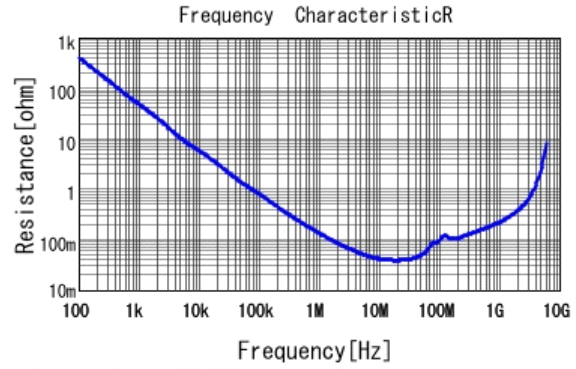
■ GCJ188R92A473MA01 R DCOV, 25degC
