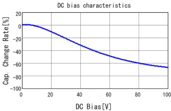
■ GCJ188R92A473MA01 C-DC bias capchange, 25.0degC, AC1.
