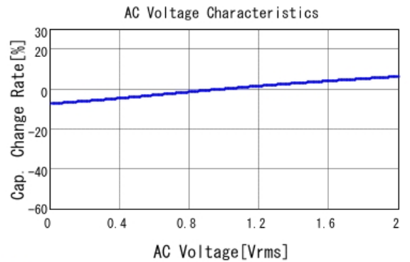
■ GCJ188R92A473MA01 C-AC Voltage capchange, DCOV, 25.0d
