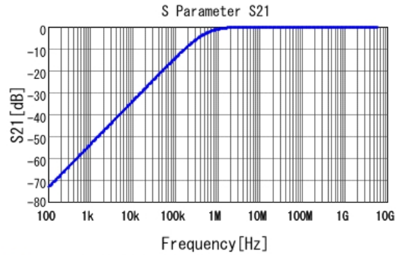
■ GCJ188R92A332KA01 S21 DC0V, 25degC
