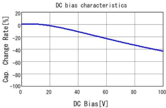
■ GCJ188R92A332KA01 C-DC bias capchange, 25.0degC, AC1.
