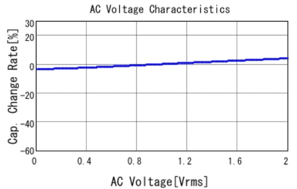
■ GCJ188R92A332KA01 C-AC Voltage capchange, DCOV, 25.0d
