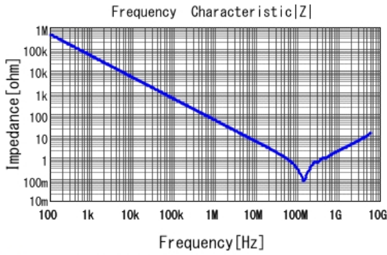
■ GCJ188R92A332KA01 |Z| DCOV, 25degC
