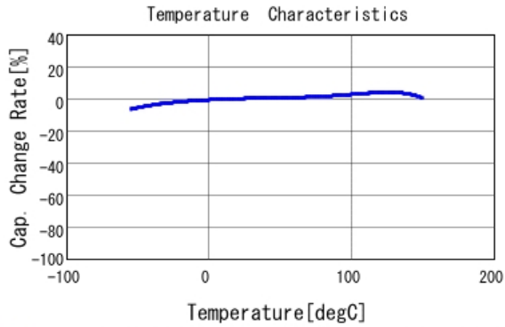
■ GCJ188R92A332KA01 C-Temp. capchange, DC0.0V, AC1.0V rm
