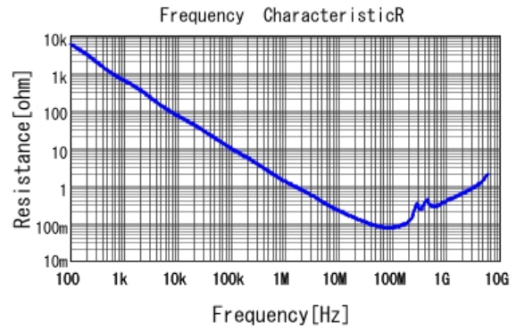
■ GCJ188R92A332KA01 R DCOV, 25degC
