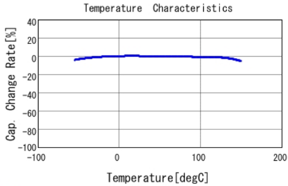
■ GCJ188R92A223KA01 C-Temp. capchange, DC0.0V, AC1.0Vrm
