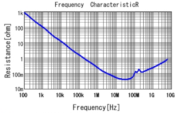
■ GCJ188R92A223KA01 R DCOV, 25degC
