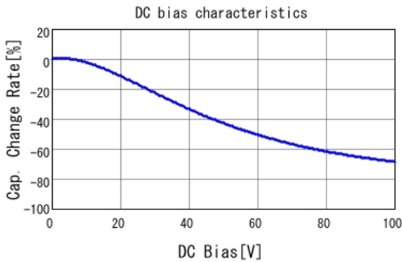
■ GCJ188R92A223KA01 C-DC bias capchange, 25.0degC, AC1.
