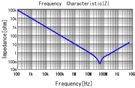
■ GCJ188R92A223KA01 |Z| DCOV, 25degC
