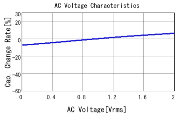
■ GCJ188R92A223KA01 C-AC Voltage capchange, DCOV, 25.0d
