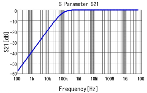
■ GCJ188R92A223KA01 S21 DC0V, 25degC
