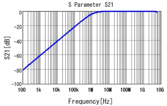
■ GCJ188R92A152KA01 S21 DC0V, 25degC
