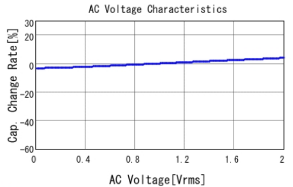
■ GCJ188R92A152KA01 C-AC Voltage capchange, DCOV, 25.0d
