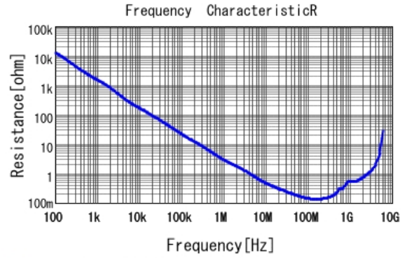
■ GCJ188R92A152KA01 R DCOV, 25degC
