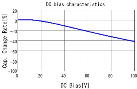
■ GCJ188R92A152KA01 C-DC bias capchange, 25.0degC, AC1.
