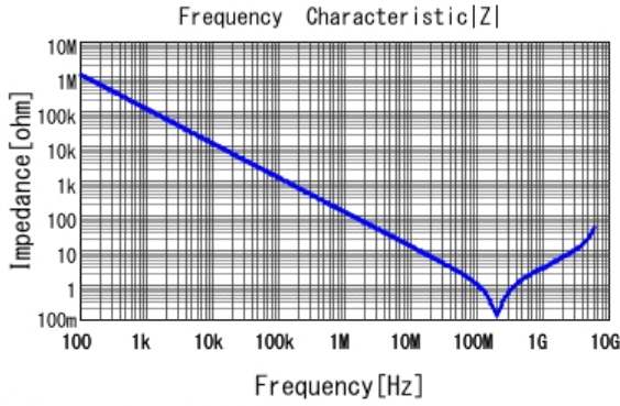
■ GCJ188R92A152KA01 |Z| DCOV, 25degC
