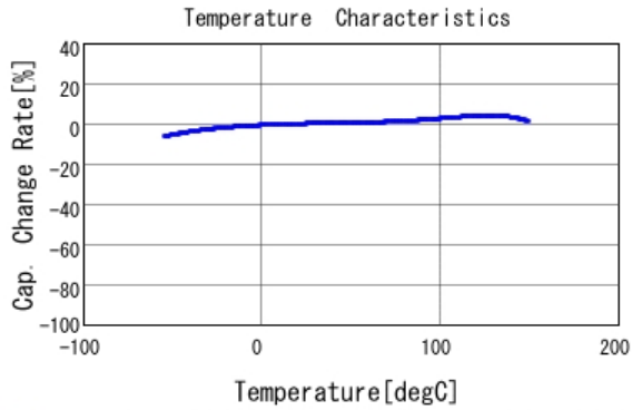
■ GCJ188R92A152KA01 C-Temp. capchange, DC0.0V, AC1.0Vrm
