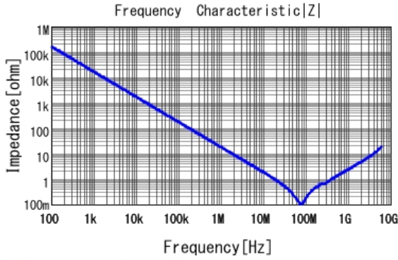
■ GCJ188R92A103KA01 |Z| DC0V, 25degC
