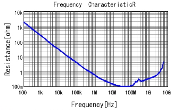
■ GCJ188R92A103KA01 R DC0V, 25degC
