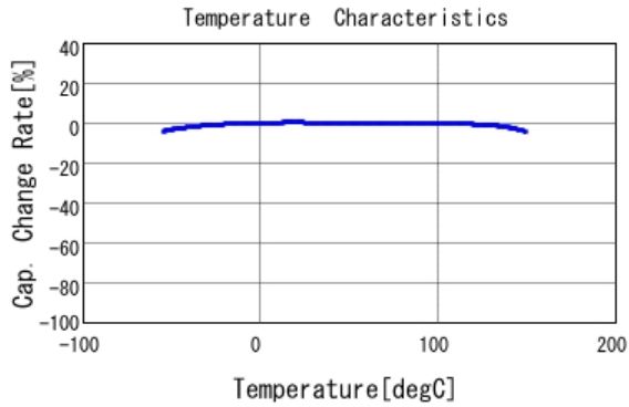
■ GCJ188R92A103KA01 C-Temp. capchange, DC0.0V, AC1.0Vrm
