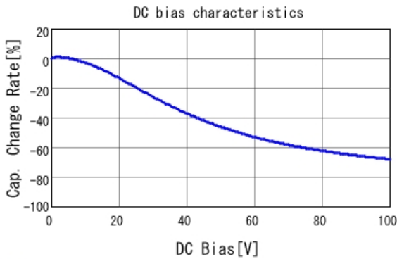
■ GCJ188R92A103KA01 C-DC bias capchange, 25.0degC, AC1.
