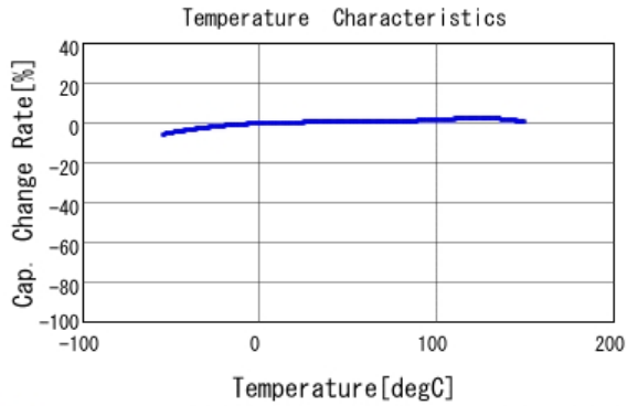
■ GCJ188R91H472KA01 C-Temp. capchange, DC0.0V, AC1.0Vrm
