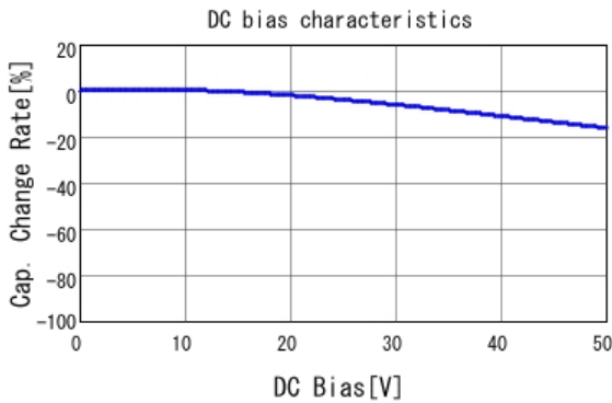
■ GCJ188R91H472KA01 C-DC bias capchange, 25.0degC, AC1.
