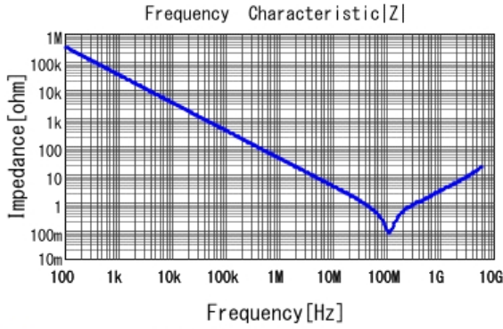
■ GCJ188R91H472KA01 |Z| DCOV, 25degC
