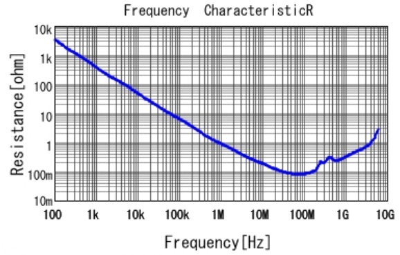
■ GCJ188R91H472KA01 R DCOV, 25degC
