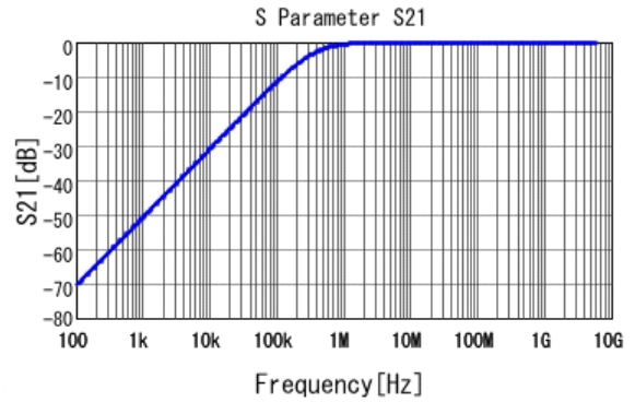
■ GCJ188R91H472KA01 S21 DC0V, 25degC
