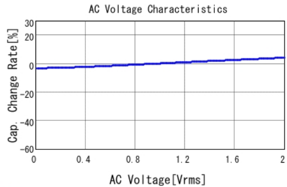
■ GCJ188R91H472KA01 C-AC Voltage capchange, DCOV, 25.0d
