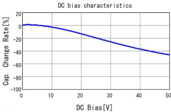
■ GCJ188R91H103KA01 C-DC bias capchange, 25.0degC, AC1.
