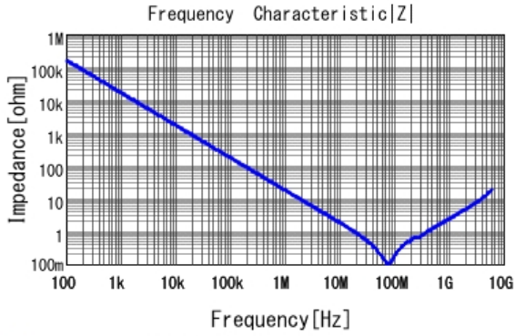
■ GCJ188R91H103KA01 |Z| DCOV, 25degC
