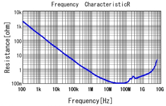
■ GCJ188R91H103KA01 R DCOV, 25degC
