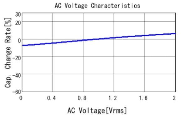
■ GCJ188R91H103KA01 C-AC Voltage capchange, DCOV, 25.0d
