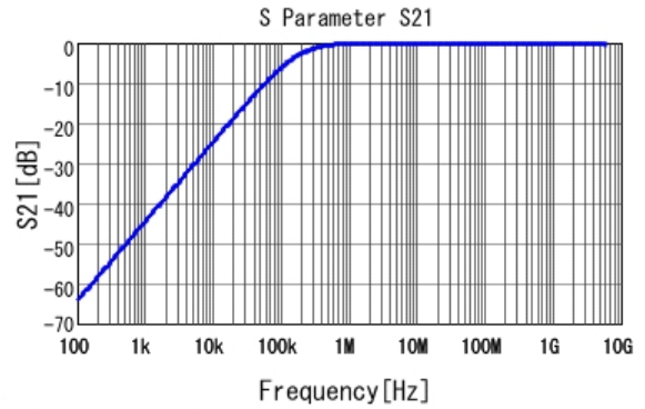
■ GCJ188R91H103KA01 S21 DC0V, 25degC
