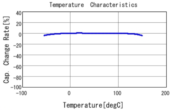
■ GCJ188R91H103KA01 C-Temp. capchange, DC0.0V, AC1.0Vrm
