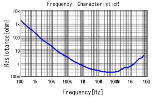
■ GCJ188R72A472KA01 R DCOV, 25degC
