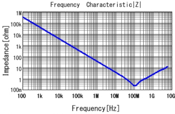
■ GCJ188R72A472KA01 |Z| DCOV, 25degC
