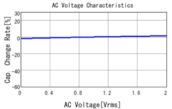
■ GCJ188R72A472KA01 C-AC Voltage capchange, DCOV, 25.0d
