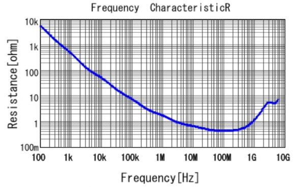
■ GCJ188R72A152KA01 R DCOV, 25degC
