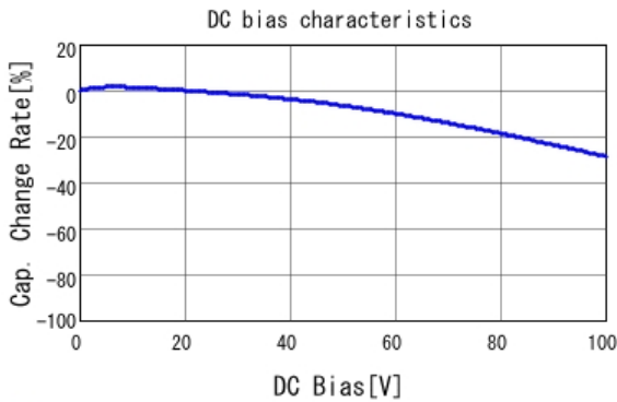
■ GCJ188R72A152KA01 C-DC bias capchange, 25.0degC, AC1.
