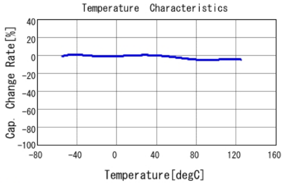
■ GCJ188R72A152KA01 C-Temp. capchange, DC0.0V, AC1.0Vrm
