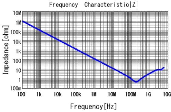
■ GCJ188R72A152KA01 |Z| DCOV, 25degC
