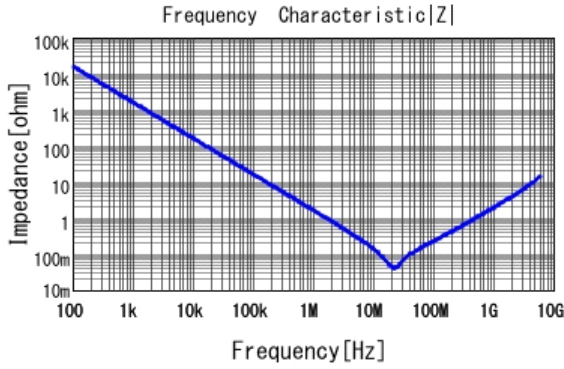
■ GCJ188R72A104MA01 |Z| DC0V, 25degC
