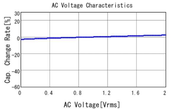
■ GCJ188R72A104MA01 C-AC Voltage capchange, DC0V, 25.0d
