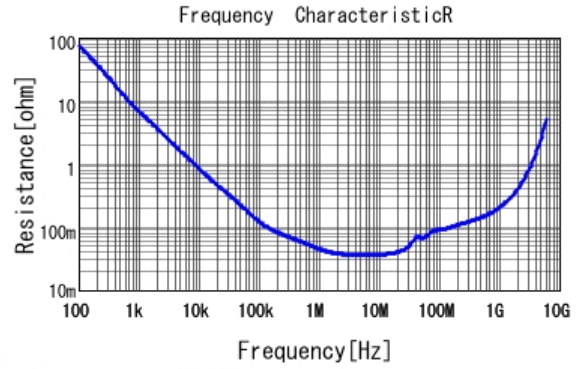
■ GCJ188R72A104MA01 R DC0V, 25degC
