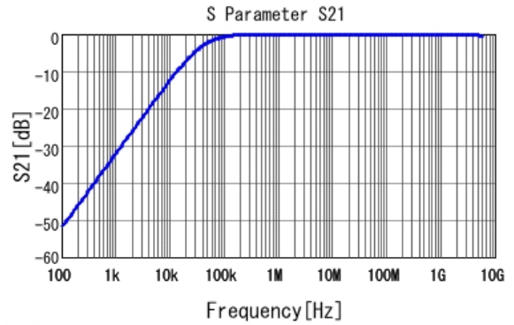
■ GCJ188R71H393KA12 S21 DC0V, 25degC
