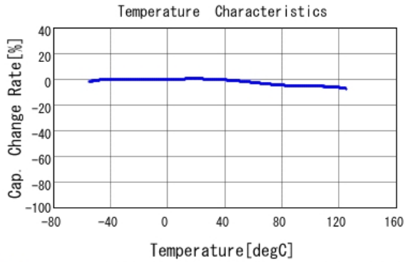
■ GCJ188R71H393KA12 C-Temp. capchange, DC0.0V, AC1.0Vrm
