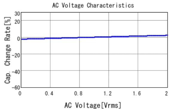
■ GCJ188R71H393KA12 C-AC Voltage capchange, DCOV, 25.0d
