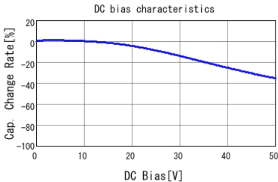
■ GCJ188R71H393KA12 C-DC bias capchange, 25.0degC, AC1.
