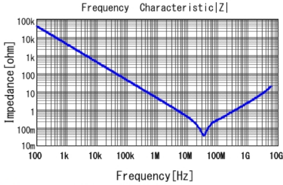
■ GCJ188R71H393KA12 |Z| DCOV, 25degC
