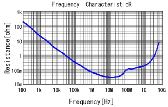
■ GCJ188R71H393KA12 R DCOV, 25degC
