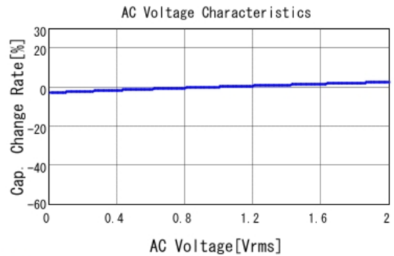
■ GCJ188R71H104MA12 C-AC Voltage capchange, DCOV, 25.0d
