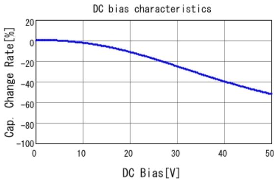
■ GCJ188R71H104MA12 C-DC bias capchange, 25.0degC, AC1.
