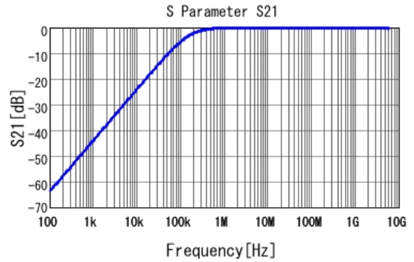
■ GCJ188R71H103MA01 S21 DC0V, 25degC
