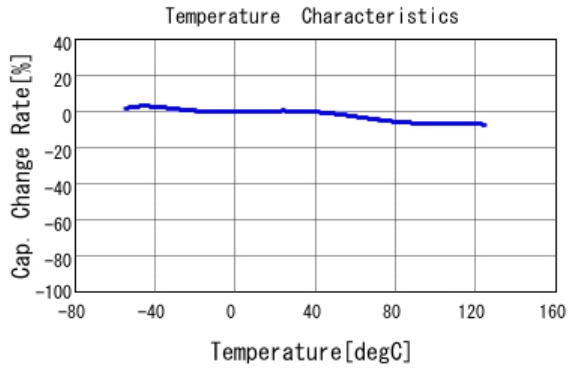
■ GCJ188R71H103MA01 C-Temp. capchange, DC0.0V, AC1.0V rm
