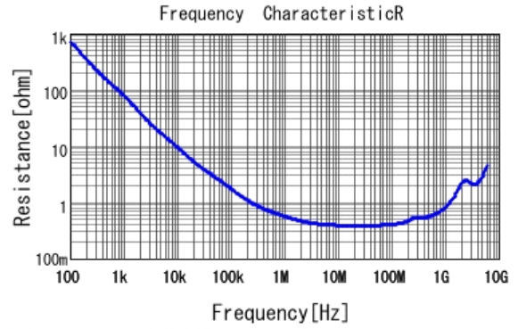
■ GCJ188R71H103MA01 R DCOV, 25degC
