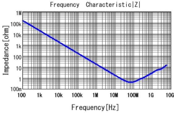
■ GCJ188R71H103MA01 |Z| DCOV, 25degC
