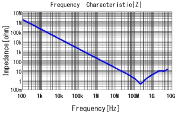
■ GCJ188R71H102MA01 |Z| DCOV, 25degC
