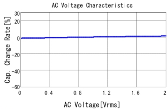
■ GCJ188R71H102MA01 C-AC Voltage capchange, DCOV, 25.0d
