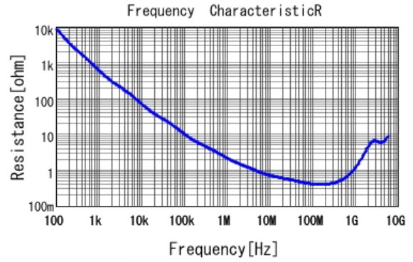
■ GCJ188R71H102MA01 R DCOV, 25degC
