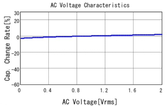
■ GCJ188R71C103KA01 C-AC Voltage capchange, DCOV, 25.0d
