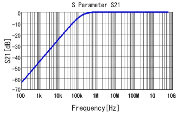
■ GCJ188R71C103KA01 S21 DC0V, 25degC
