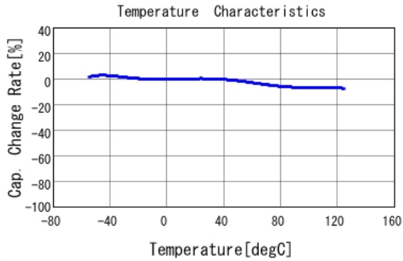
■ GCJ188R71C103KA01 C-Temp. capchange, DC0.0V, AC1.0Vrm
