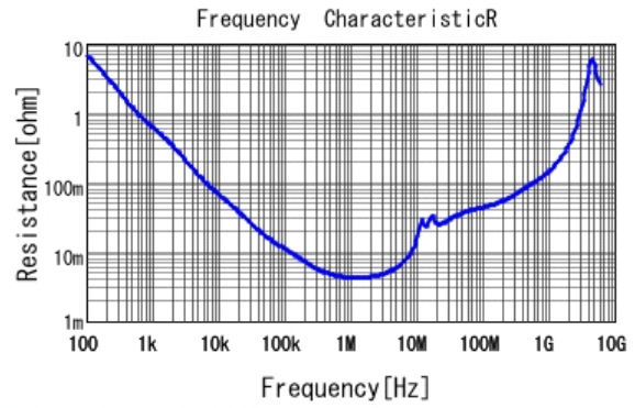
GCH21BR71H105KE01 R DC0V, 25degC
