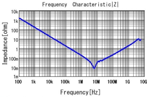
GCH21BR71H105KE01 |Z| DC0V, 25degC
