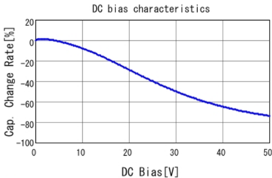
GCH21BR71H105KE01 C-DC bias capchange, 25.0degC, AC1.
