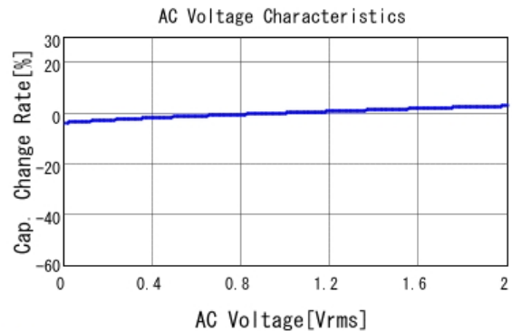
GCH21BR71H105KE01 C-AC Voltage capchange, DC0V, 25.0d
