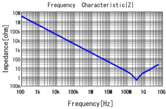
■ GCE219R72A471KA01 |Z| DC0V, 25degC
