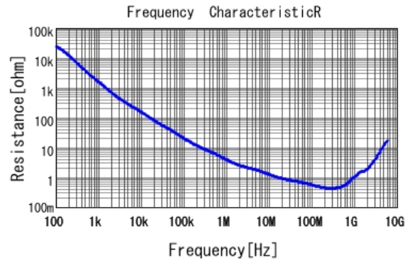
■ GCE219R72A471KA01 R DC0V, 25degC
