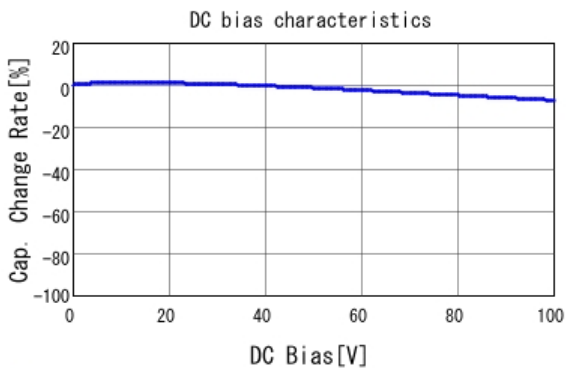
■ GCE219R72A471KA01 C-DC bias capchange, 25.0degC, AC1.
