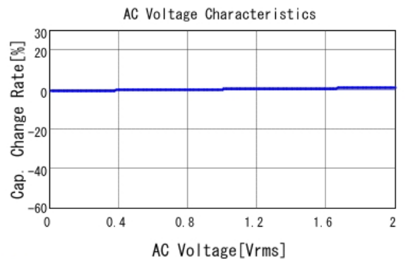
■ GCE219R72A471KA01 C-AC Voltage capchange, DC0V, 25.0d
