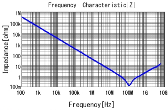
■ GCE188R72A472KA01 |Z| DCOV, 25degC
