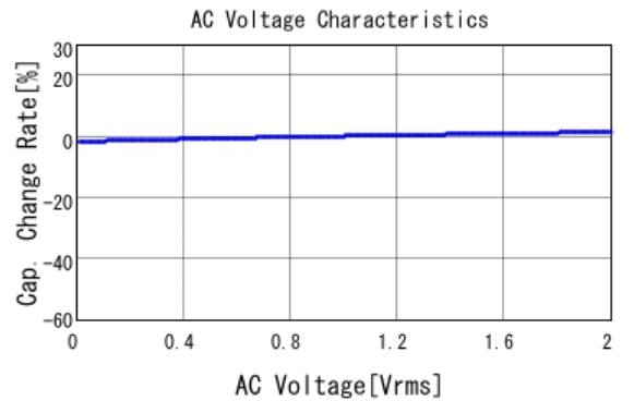
■ GCE188R72A472KA01 C-AC Voltage capchange, DCOV, 25.0d
