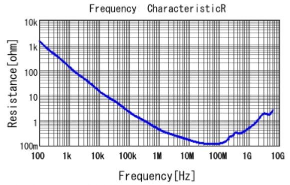
■ GCE188R72A472KA01 R DCOV, 25degC
