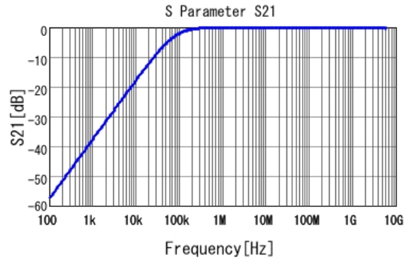
■ GCE188R72A223KA01 S21 DC0V, 25degC
