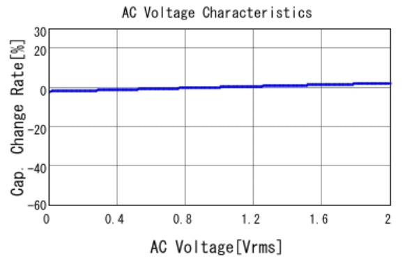
■ GCE188R72A223KA01 C-AC Voltage capchange, DCOV, 25.0d
