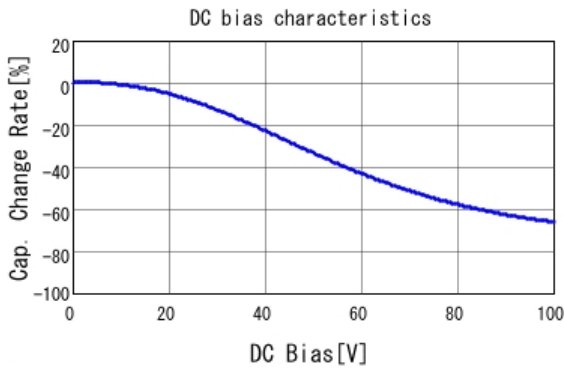
■ GCE188R72A223KA01 C-DC bias capchange, 25.0degC, AC1.
