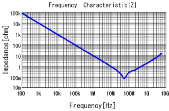
■ GCE188R72A223KA01 |Z| DCOV, 25degC
