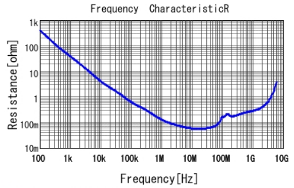
■ GCE188R72A223KA01 R DCOV, 25degC
