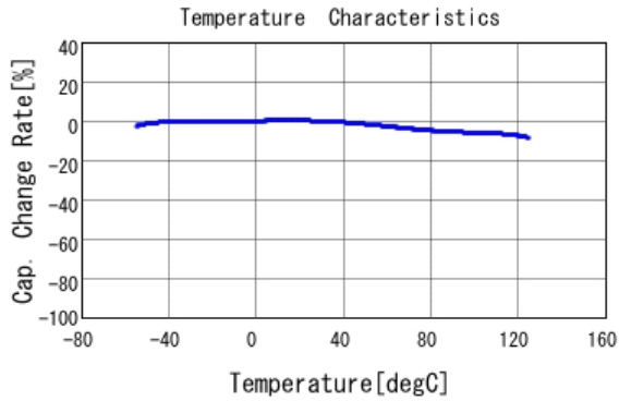
■ GCE188R72A223KA01 C-Temp. capchange, DC0.0V, AC1.0Vrm
