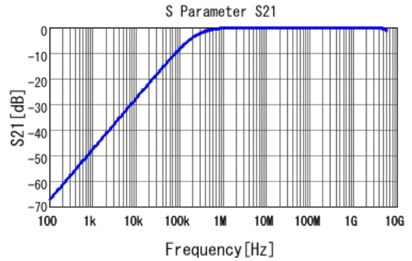
■ GCE188R71H682KA01 S21 DC0V, 25degC
