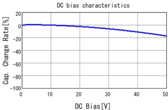
■ GCE188R71H682KA01 C-DC bias capchange, 25.0degC, AC1.
