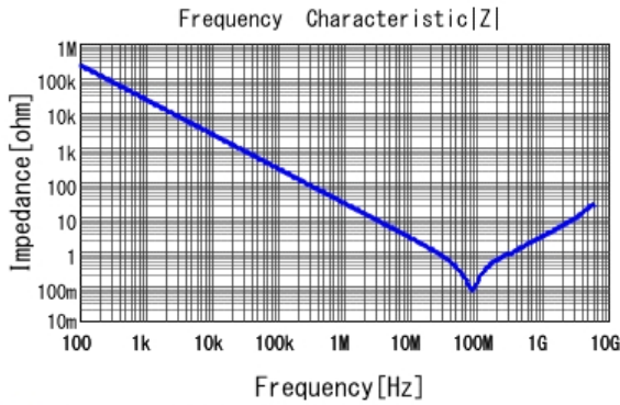
■ GCE188R71H682KA01 |Z| DCOV, 25degC
