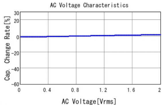
■ GCE188R71H682KA01 C-AC Voltage capchange, DCOV, 25.0d
