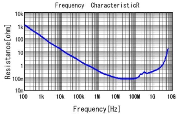
■ GCE188R71H682KA01 R DCOV, 25degC
