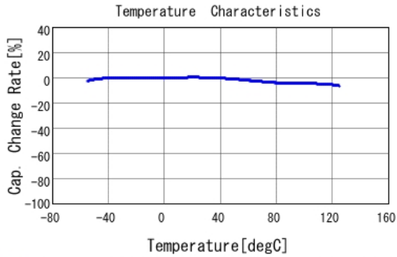
■ GCE188R71H682KA01 C-Temp. capchange, DC0.0V, AC1.0Vrm
