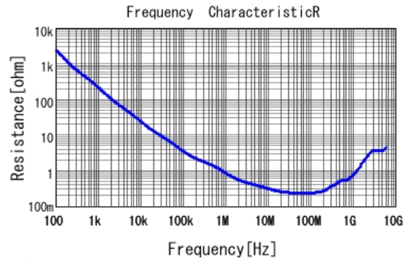
■ GCE188R71H332KA01 R DCOV, 25degC
