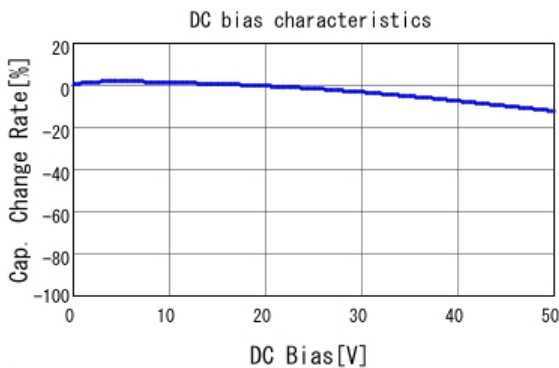
■ GCE188R71H332KA01 C-DC bias capchange, 25.0degC, AC1.
