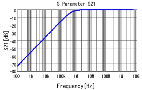
■ GCE188R71H332KA01 S21 DC0V, 25degC
