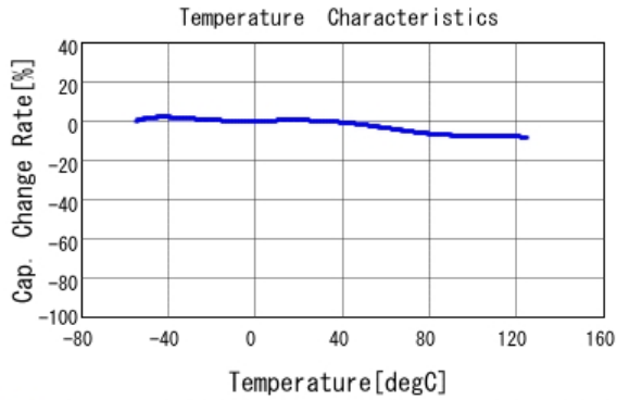
■ GCE188R71H332KA01 C-Temp. capchange, DC0.0V, AC1.0Vrm
