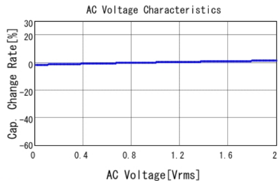
■ GCE188R71H332KA01 C-AC Voltage capchange, DCOV, 25.0d
