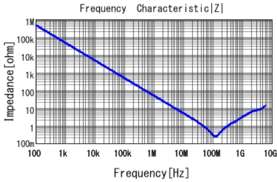
■ GCE188R71H332KA01 |Z| DCOV, 25degC
