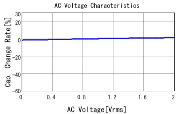
■ GCE188R71H222KA01 C-AC Voltage capchange, DCOV, 25.0d
