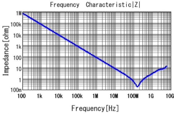
■ GCE188R71H222KA01 |Z| DCOV, 25degC
