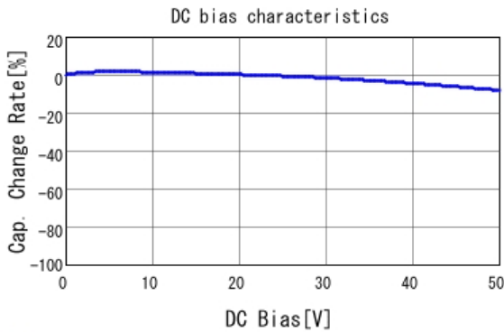
■ GCE188R71H222KA01 C-DC bias capchange, 25.0degC, AC1.
