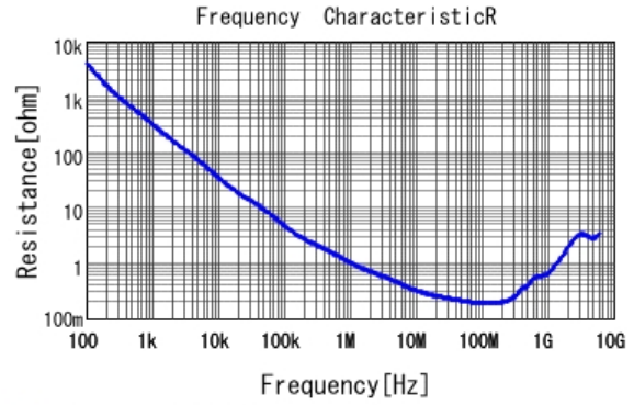
■ GCE188R71H222KA01 R DCOV, 25degC
