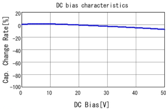
■ GCE188R71H102MA01 C-DC bias capchange, 25.0degC, AC1.
