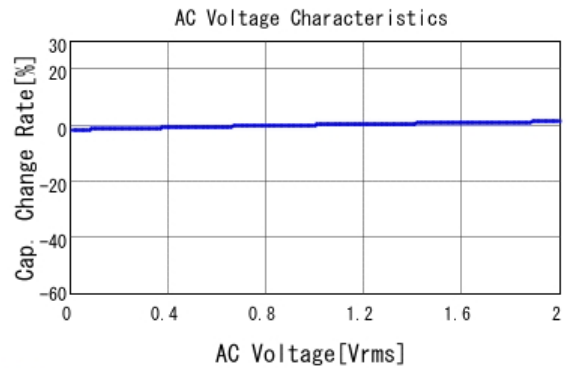
■ GCE188R71H102MA01 C-AC Voltage capchange, DCOV, 25.0d
