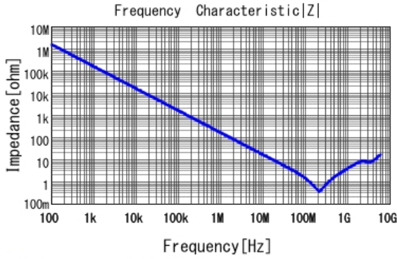
■ GCE188R71H102MA01 |Z| DCOV, 25degC
