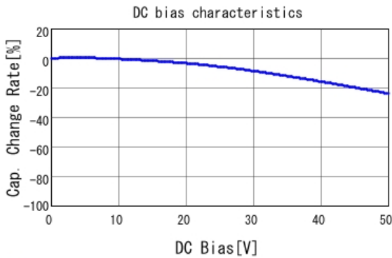
■ GCD21BR71H333MA01 C-DC bias capchange, 25.0degC, AC1.
