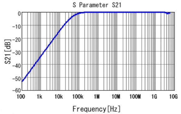
■ GCD21BR71H333MA01 S21 DC0V, 25degC
