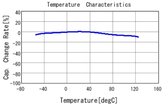
■ GCD21BR71H333MA01 C-Temp. capchange, DC0.0V, AC1.0Vrm
