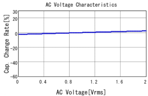
■ GCD21BR71H333MA01 C-AC Voltage capchange, DCOV, 25.0d
