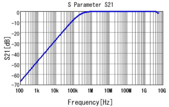
■ GCD188R72A682KA01 S21 DC0V, 25degC
