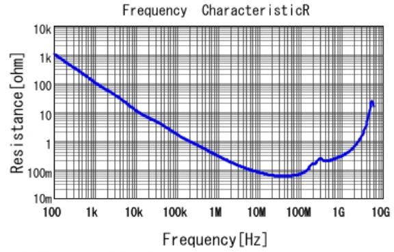
■ GCD188R72A682KA01 R DCOV, 25degC
