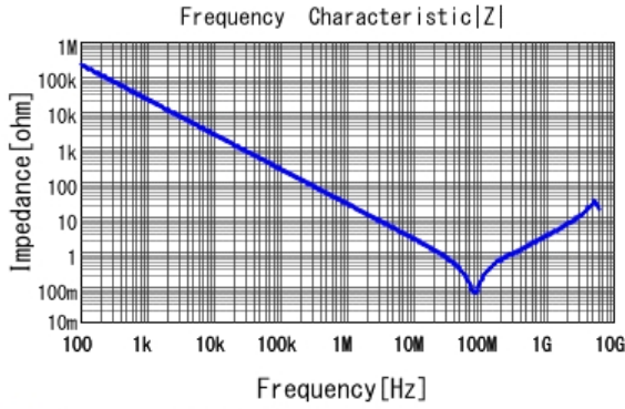
■ GCD188R72A682KA01 |Z| DCOV, 25degC
