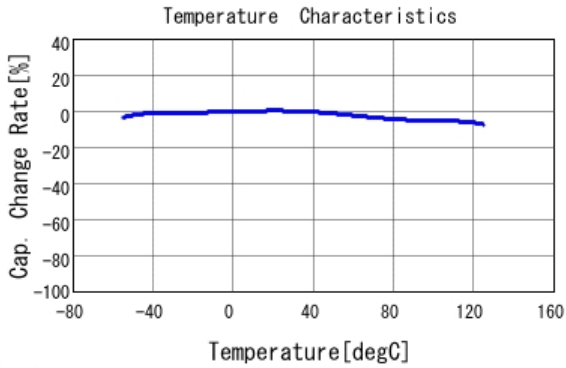
■ GCD188R72A682KA01 C-Temp. capchange, DC0.0V, AC1.0Vrm
