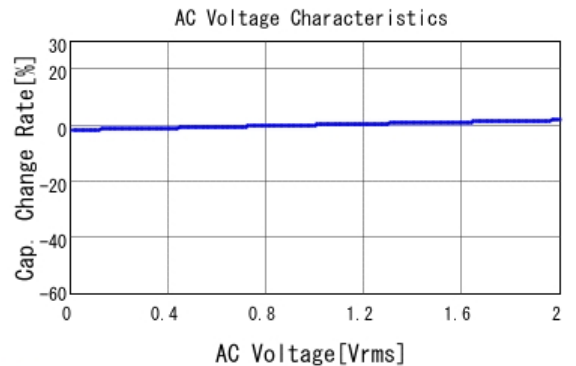
■ GCD188R72A682KA01 C-AC Voltage capchange, DCOV, 25.0d
