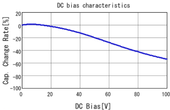
■ GCD188R72A682KA01 C-DC bias capchange, 25.0degC, AC1.
