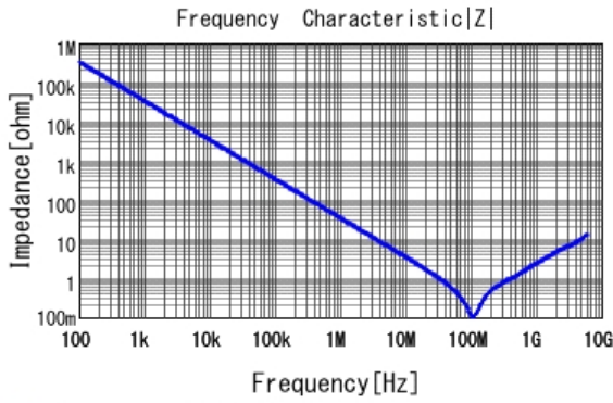
GCD188R72A472KA01 |Z| DCOV, 25degC
