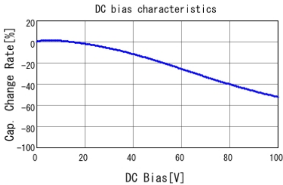
■ GCD188R72A103KA01 C-DC bias capchange, 25.0degC, AC1.
