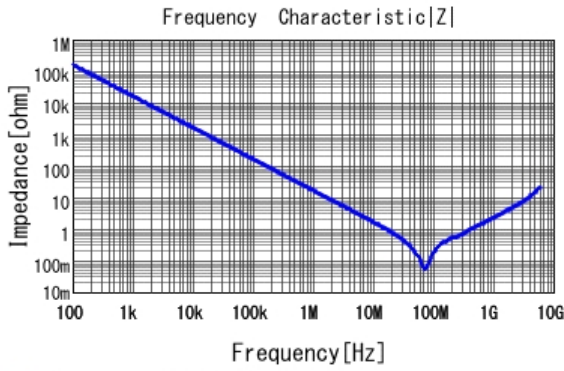
■ GCD188R72A103KA01 |Z| DCOV, 25degC
