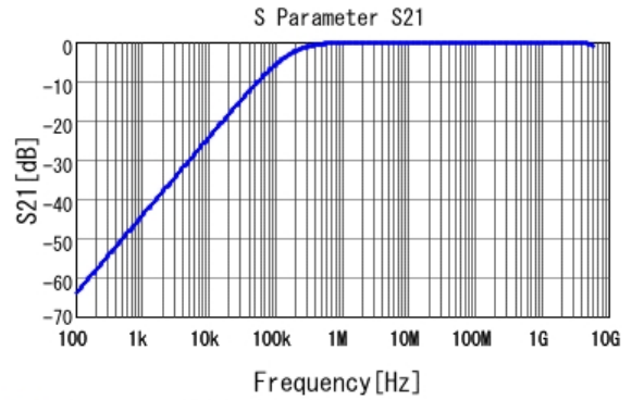
■ GCD188R72A103KA01 S21 DC0V, 25degC
