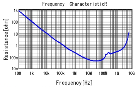
■ GCD188R72A103KA01 R DCOV, 25degC
