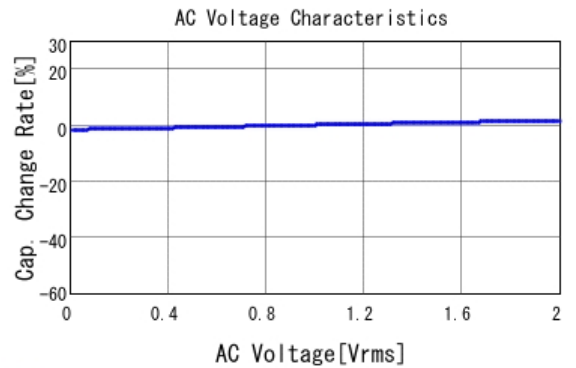
■ GCD188R72A103KA01 C-AC Voltage capchange, DCOV, 25.0d
