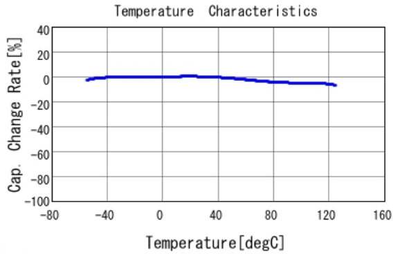
■ GCD188R72A103KA01 C-Temp. capchange, DC0.0V, AC1.0Vrm
