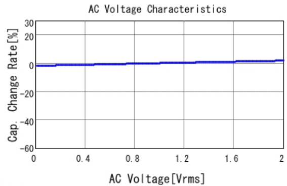
■ GCD188R71H822KA01 C-AC Voltage capchange, DCOV, 25.0d
