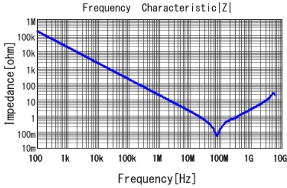
■ GCD188R71H822KA01 |Z| DCOV, 25degC
