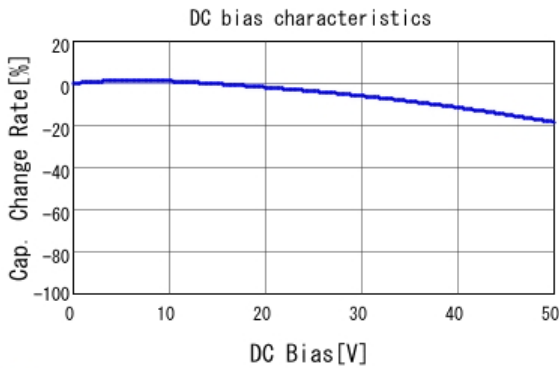
■ GCD188R71H822KA01 C-DC bias capchange, 25.0degC, AC1.
