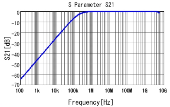
■ GCD188R71H822KA01 S21 DC0V, 25degC
