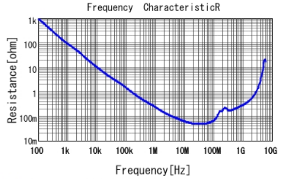
■ GCD188R71H822KA01 R DCOV, 25degC
