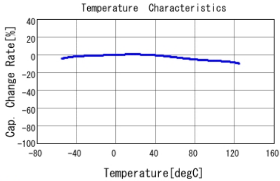
■ GCD188R71H822KA01 C-Temp. capchange, DC0.0V, AC1.0Vrm
